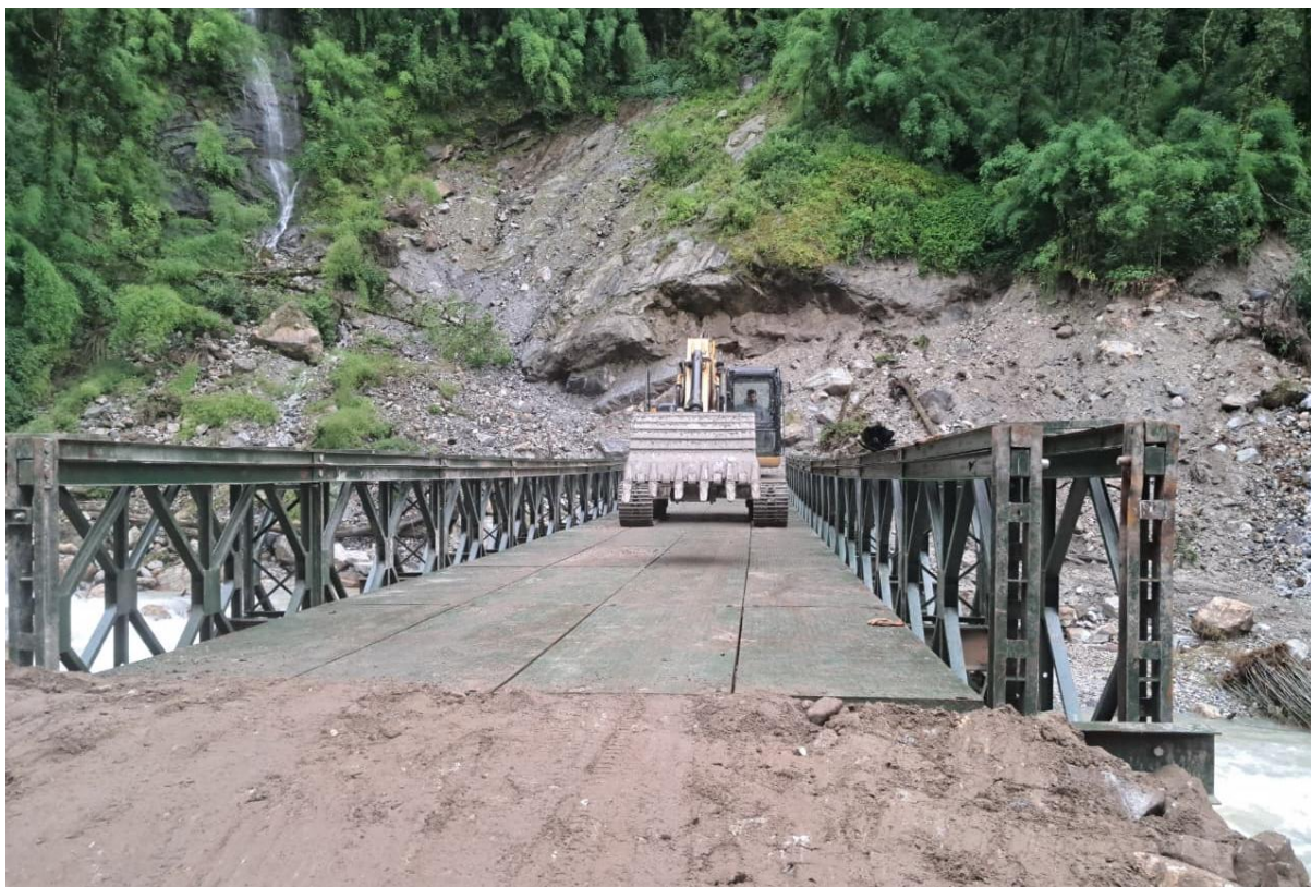
Figure 11: Bailey bridge load test by excavator
